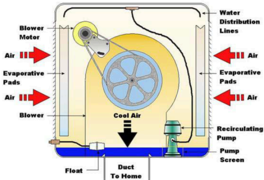
Figure 1: The general operation of the swamp cooler.
